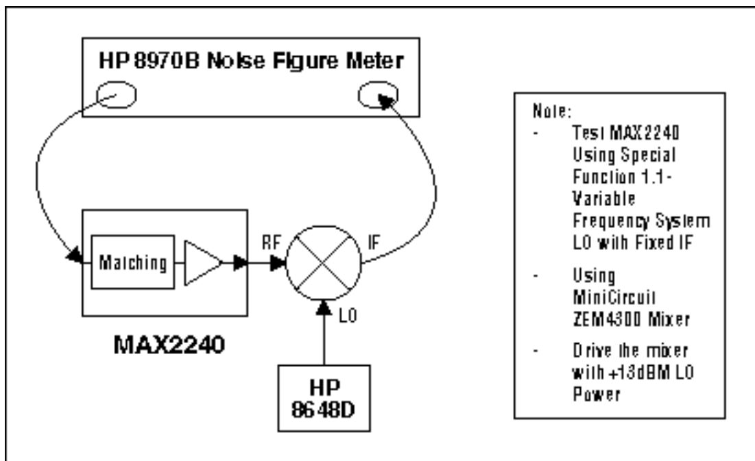
Figure 4. Bench setup for noise-figure measurements
