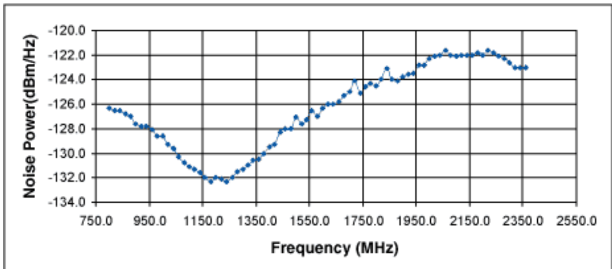
Figure 12. Noise-power-measurement graph
