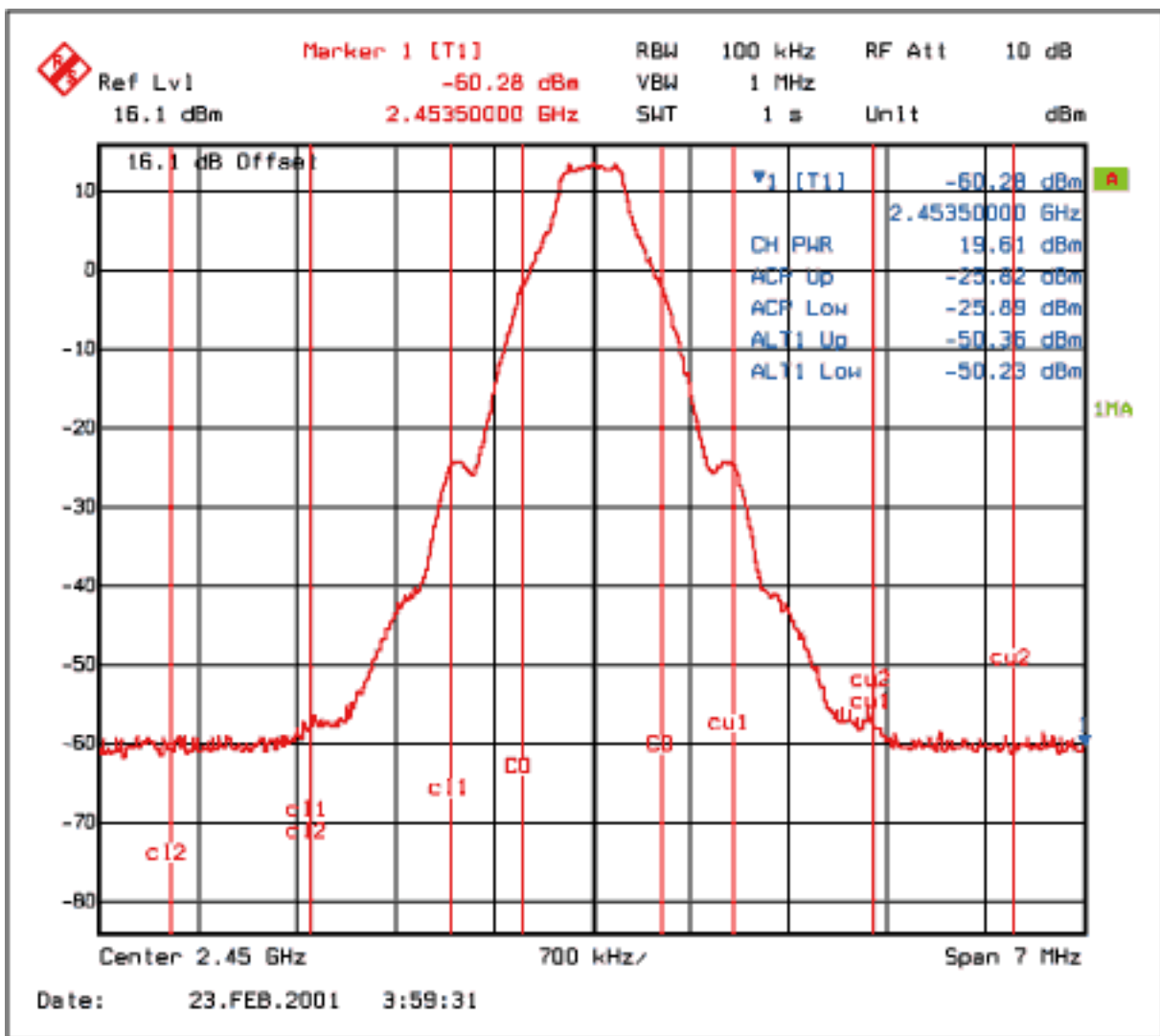
Figure 5. Maximum output at 2.45GHz with 4dBm input power, with Vcc = 3.2 volts
